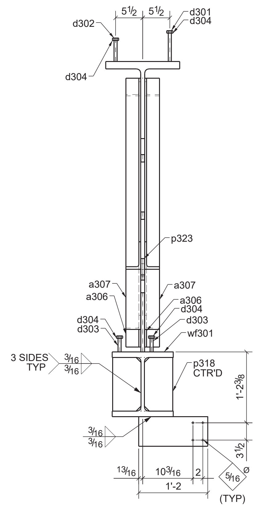
SECTION P - P
