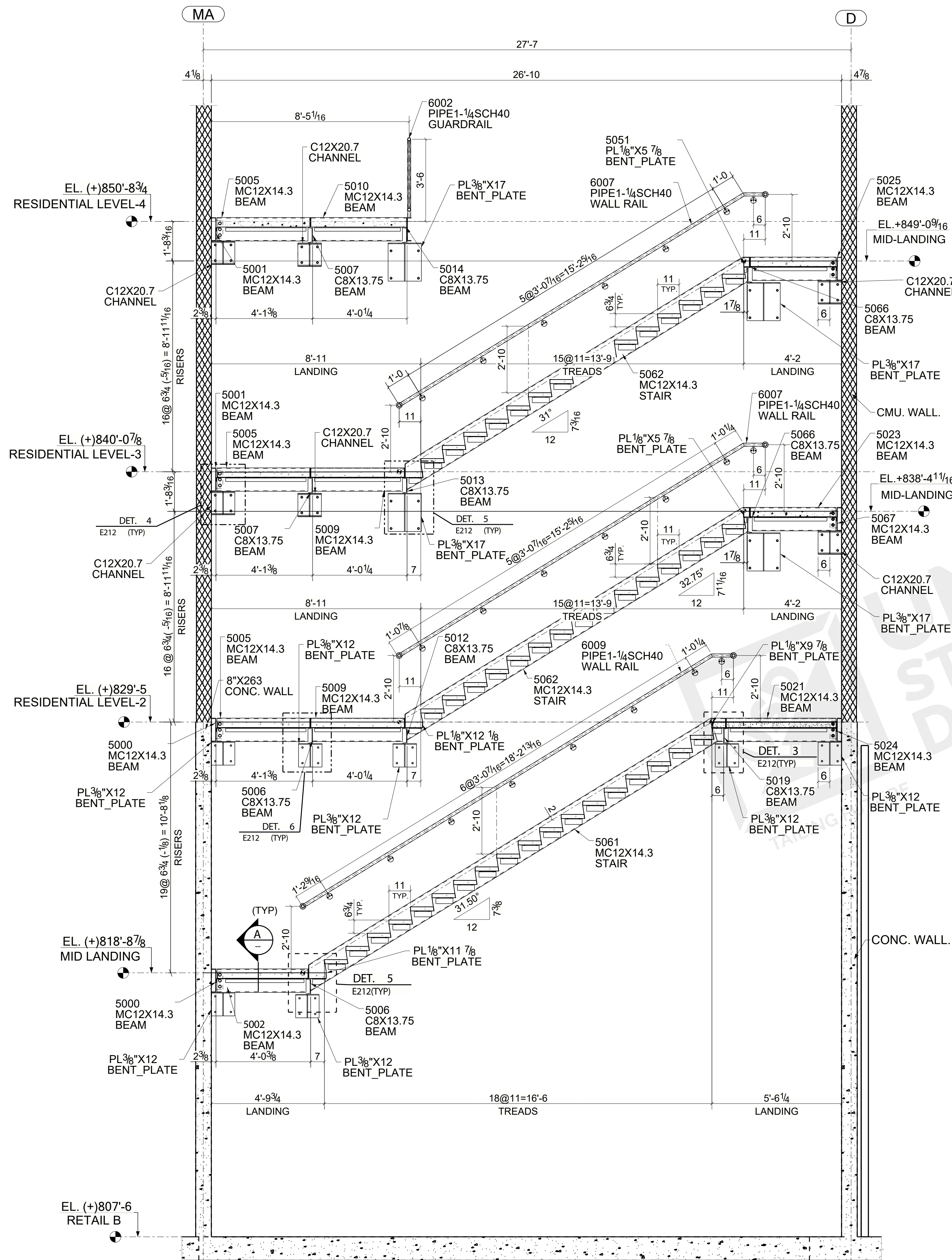
SECTION A - A (REF. DWG. NO: 1/ A6.01)
