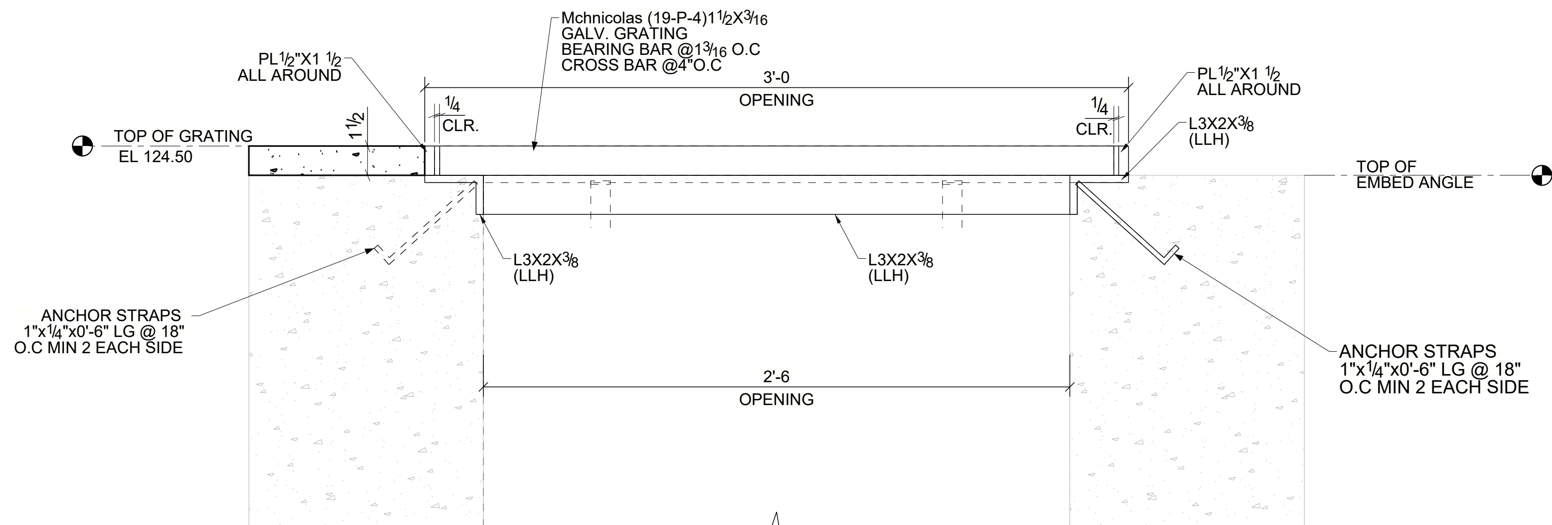
SECTION A - A (REF :- C/S-CD-703 & 3/ S-WP-101)
